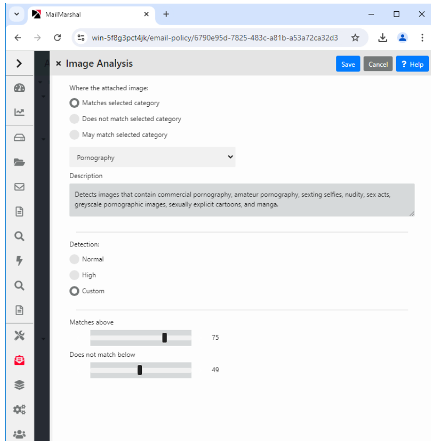
Figure 13: Image analysis rule condition
