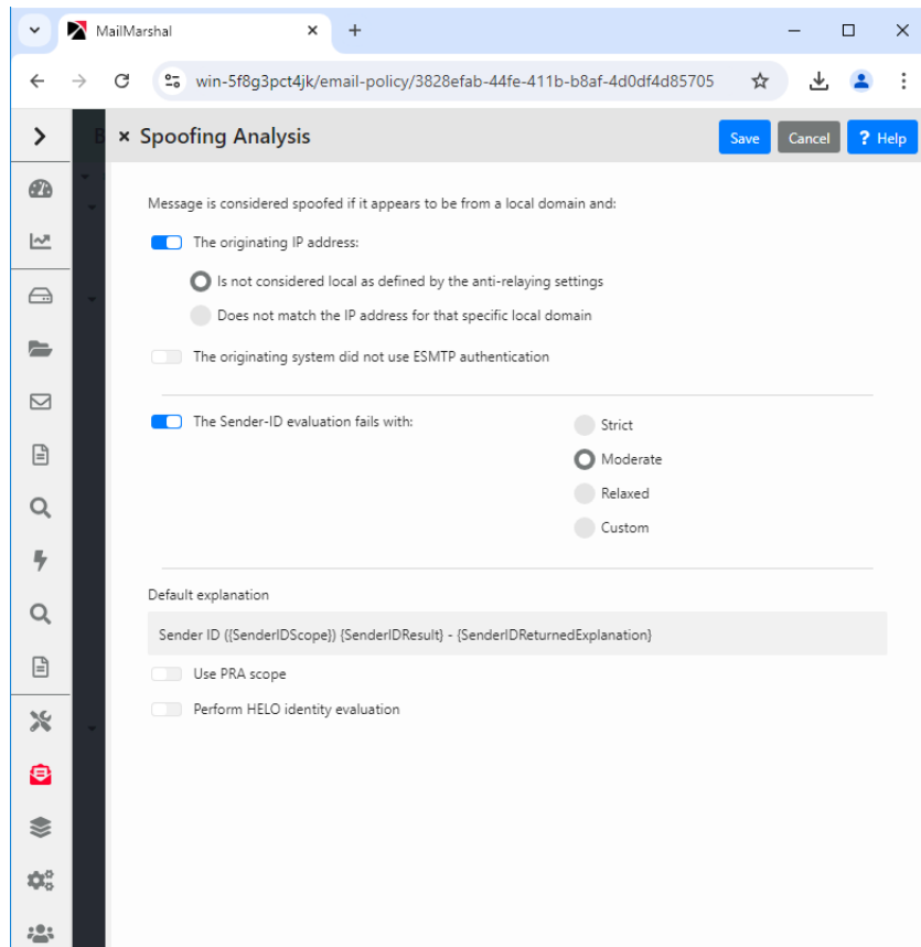
Figure 12: Message spoofing analysis rule condition
