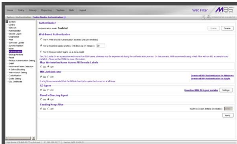
Fig. A-3 Enable/Disable Authentication window, AD Agent frame
