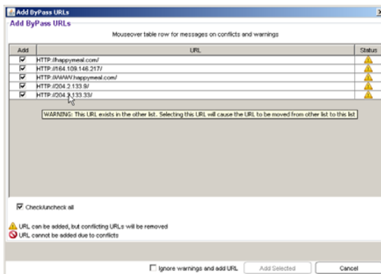
Fig. 4-10 Conflicting URLs found by query
