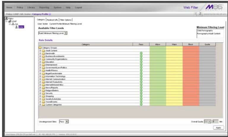
Fig. 4-5 Group Profile window, Category tab, LDAP group
