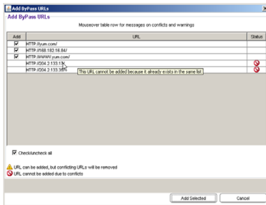
Fig. 4-9 Add ByPass URLs pop-up window
