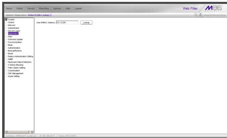
Fig. 4-15 Active Profile Lookup window
