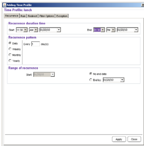
Fig. 4-14 Time Profile window Recurrence tab
