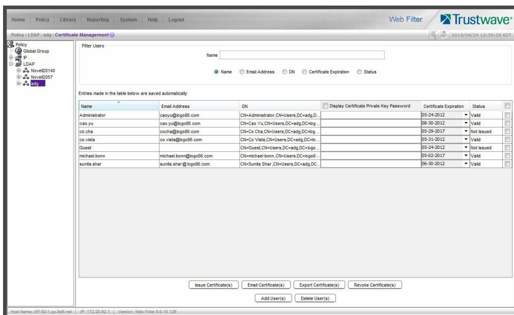
Figure 22: Certificate Management window with LDAP users imported
