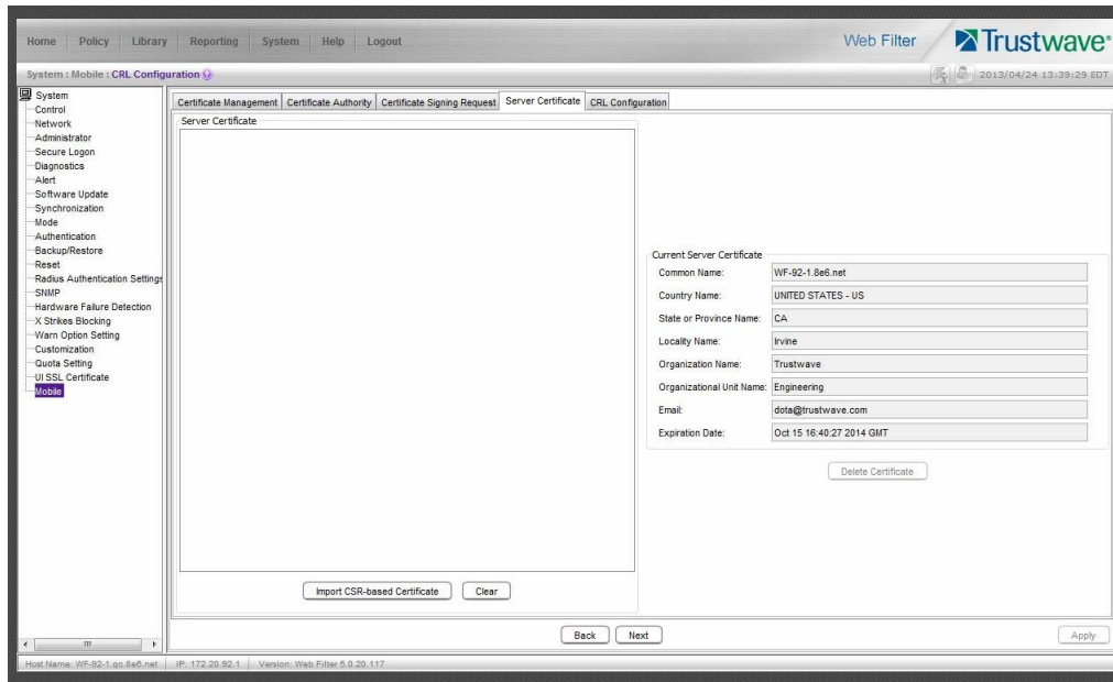
Figure 32: Current Server Certificate frame populated
