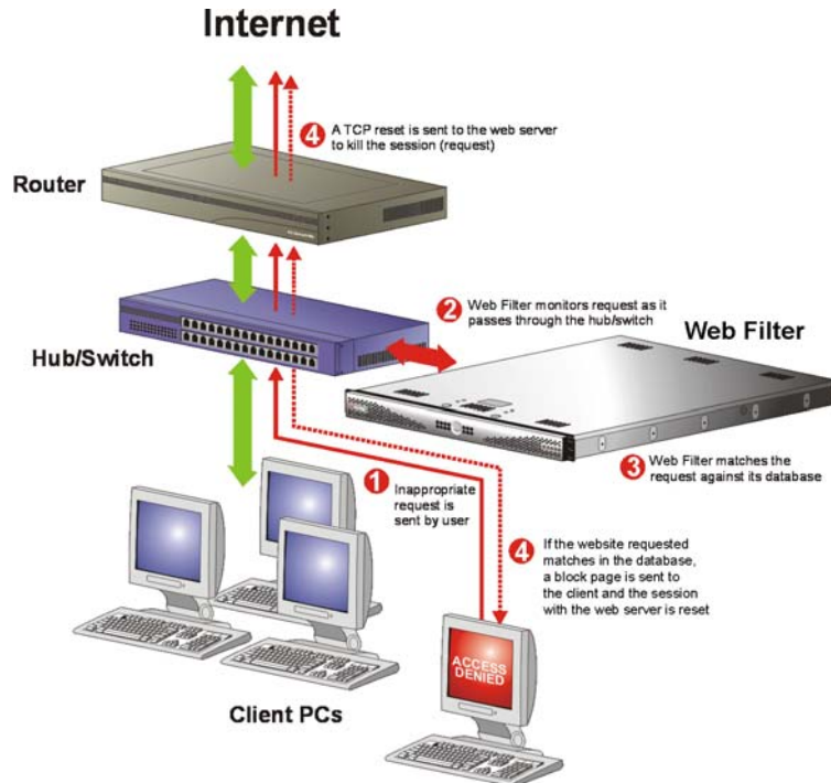
Fig. 1:1-1 Pass-by filtering diagram
