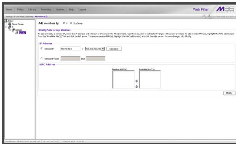
Fig. 3:1-34 Members window
