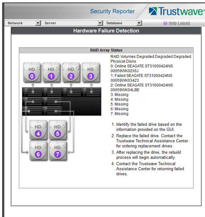
Figure 6: Hardware Failure Detection screen, 705 or 735 IBM model
