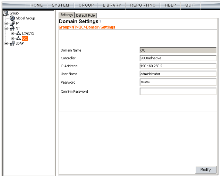
Fig. 3-2 NT Domain Details window, Settings tab
