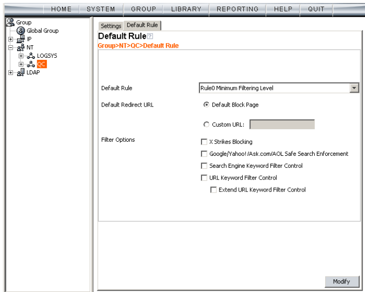
Fig. 3-3 NT Domain Details window, Default Rule tab
