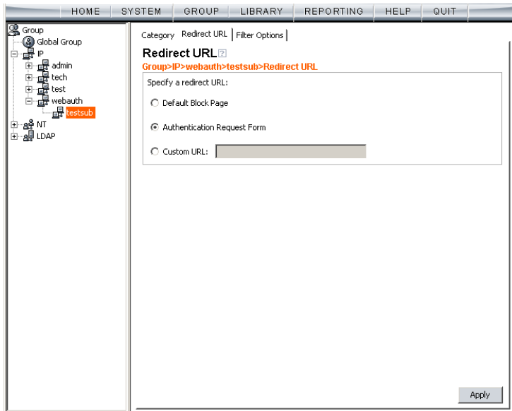
Fig. 6-16 Sub Group Profile window, Redirect URL tab
