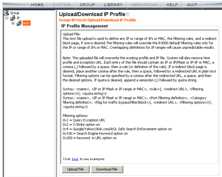
Fig. E:2-6 Master IP group's Upload/Download IP Profile window
