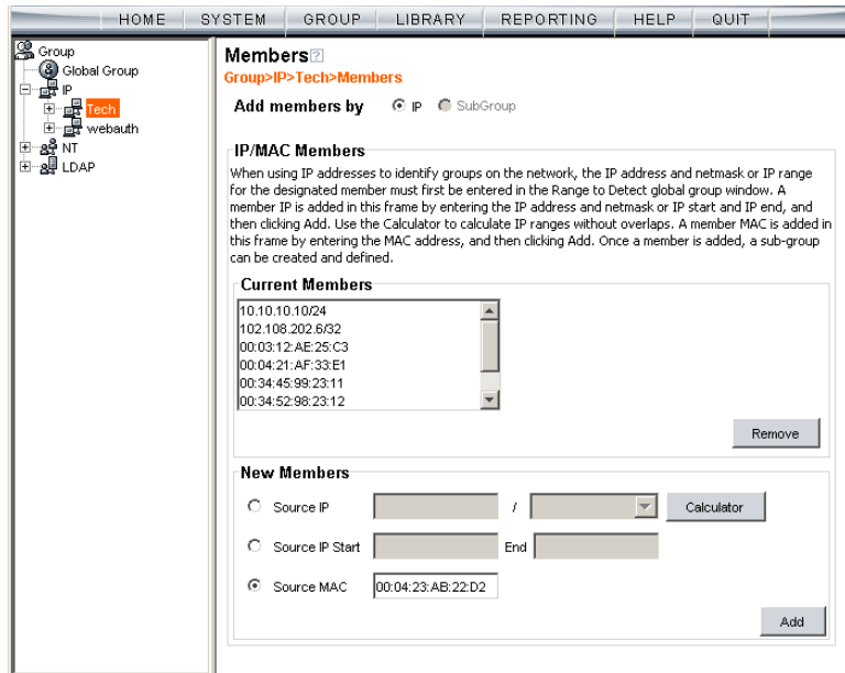
Fig. E:2-2 Members window, master IP group with MAC addresses
