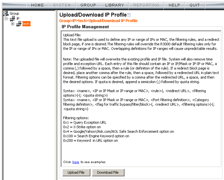
Fig. 3:1-21 Upload/Download IP Profile window
